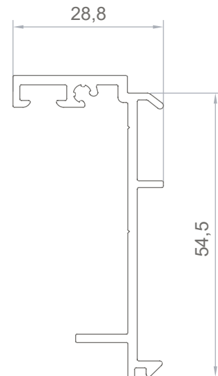
Code: PS-1580 0,555 kg/m Sash & Frame Adapter Profile
