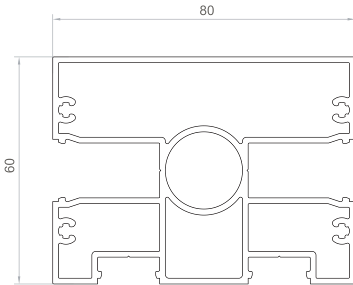
Code: PS-1581 2,231 kg/m Mullion Profile
