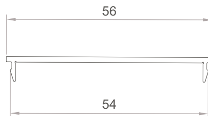
Code: ALS9460 0,255 kg/m Frame/Sash/Column Cover Profile
