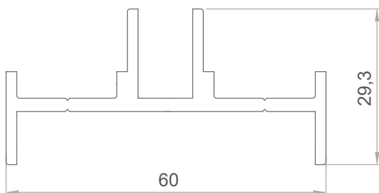
Code: PS-1058 0,805 kg/m Sash & Lamella Adapter Profile
