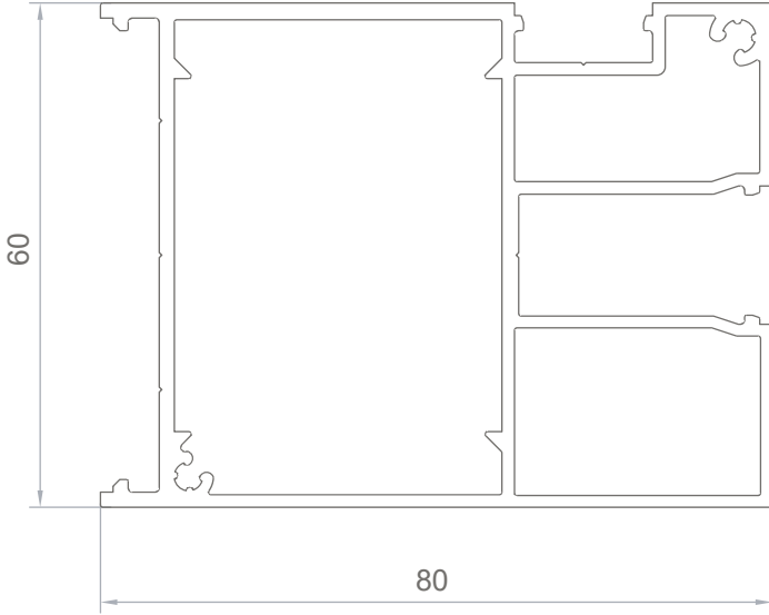
Code: PS-1578 1,787 kg/m Sash Profile
