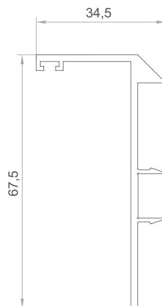
Code: PS-1107 0,589 kg/m Double Sash Stopper Profile
