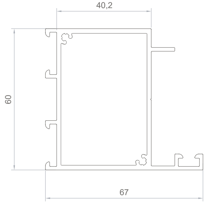
Code: PS-1579 1,333 kg/m Frame Profile
