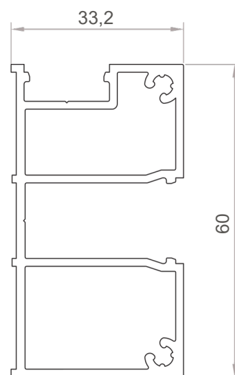
Code: PS-1587 1,068 kg/m Wall to Wall Fence Adapter Profile
